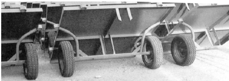
Figure 28: Two-wheel carts using roller bearings and factory-reject car tires. Designed for a team of oxen, but a smaller size is used with donkeys in Togo.
