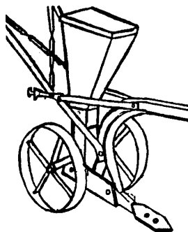
Figure 44: Ripper-planter attachment to the common plough.
