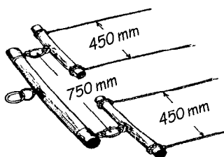
Figure 22: Suggested sizes for the swingle trees and evener.
