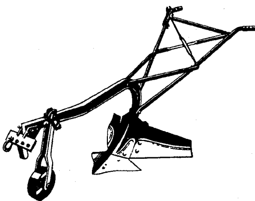
Figure 39: "Inkunki" high wing ridger, manufactured in Zimbabwe.
