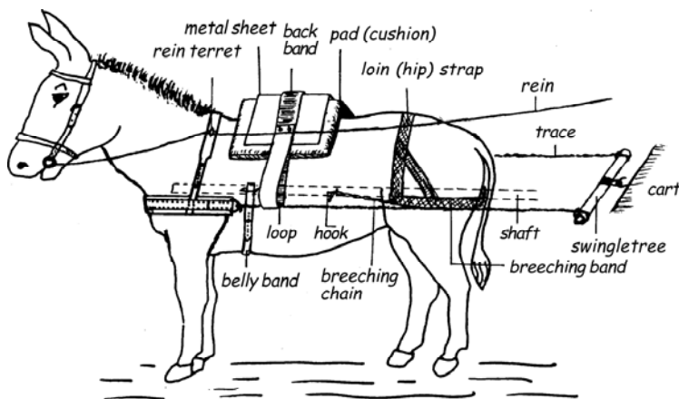
Figure 23: The arrangement of the breast band, breech strap and saddle for harnessing a donkey to the shafts of a two-wheeled cart.
