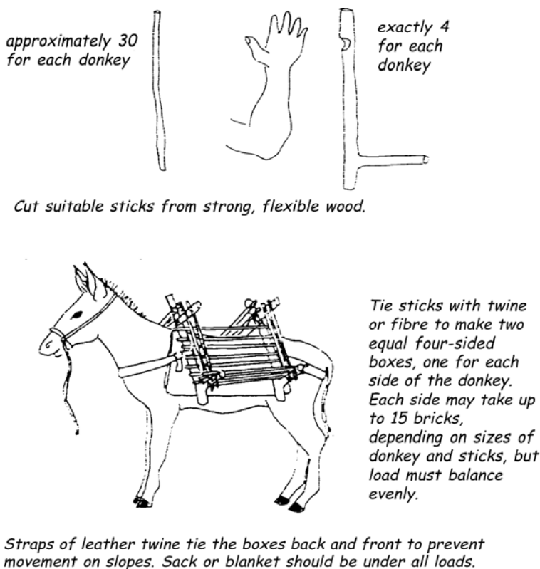
Figure 9: Simple pack frame or back-box.
