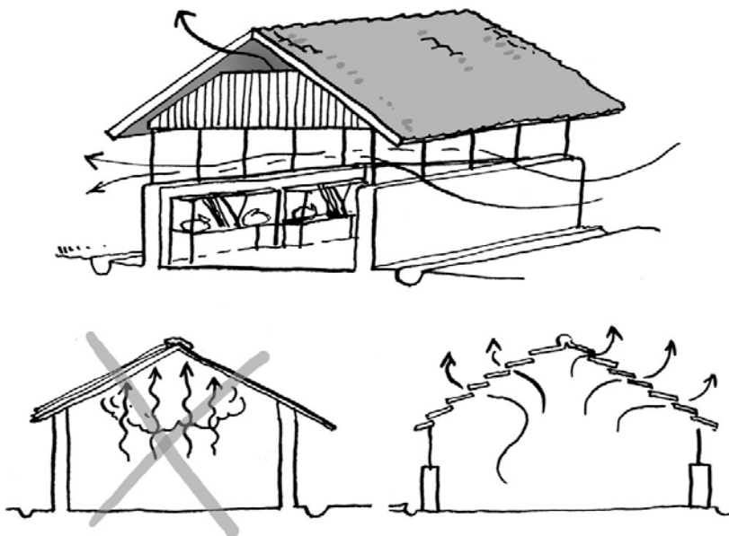
Figure 19: Roof construction in relation to ventilation
