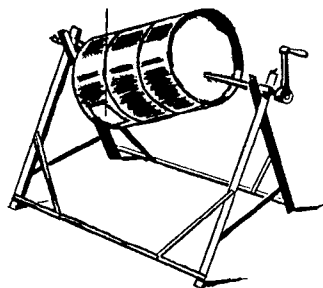
Figure 8: Hand machine for mixing
