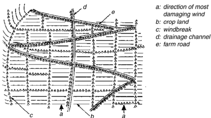
Figure 35: Siting of windbreaks.
