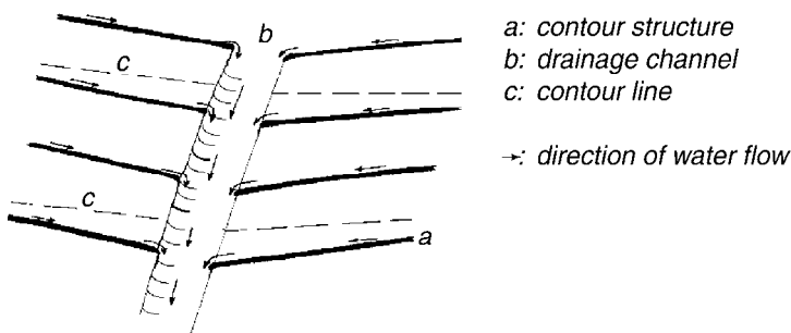
Figure 8: Drainage of a contour structure.
